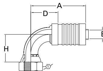
SAE 37° (JIC) 90° Elbow FC5503
