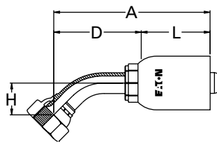
SAE 37° (JIC) Swivel 45° Elbow
