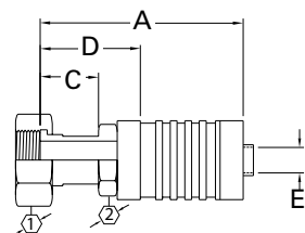
ORS Swivel Straight FJ9718
