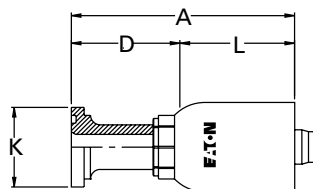
Straight Split Flange Code 61
