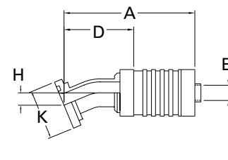
22 1/2° Elbow Split Flange FC5507 Code 61
