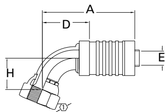
SAE 37° (JIC) 67 1/2° Elbow FJ9031
